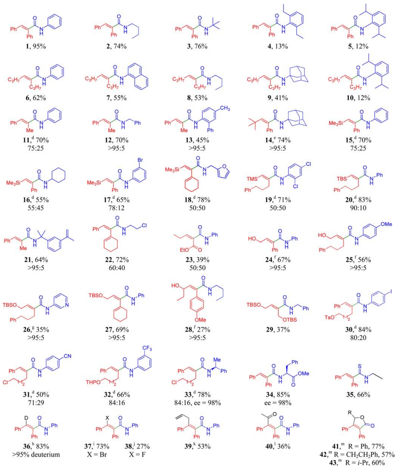
Scheme 1. \alpha,\beta -Unsaturated Amide Substrate Scope,
